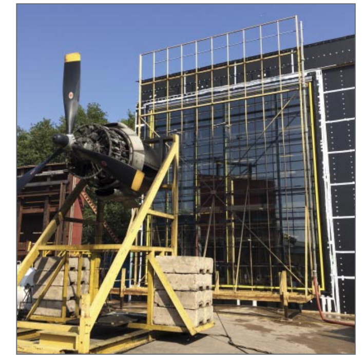
CWCT Dynamic Test
