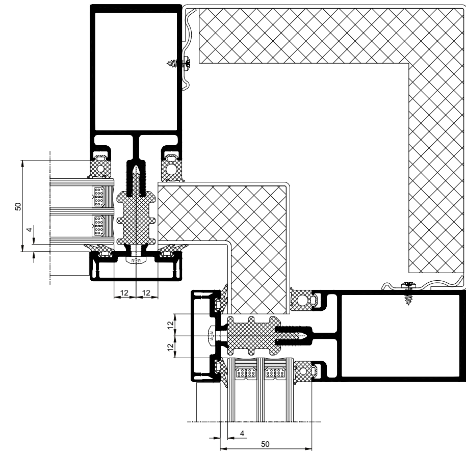
Internal Corner
