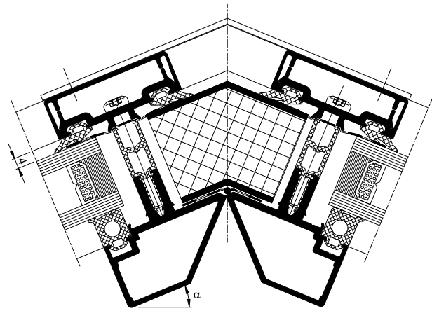
Apex (Generic)
