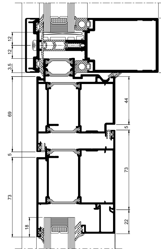
H3 10.01
