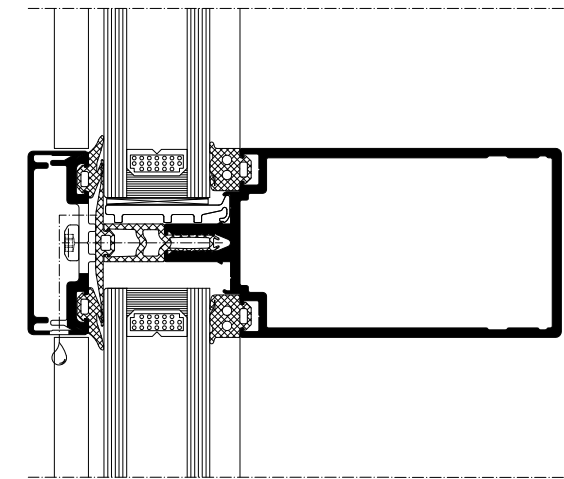
Transom Detail
