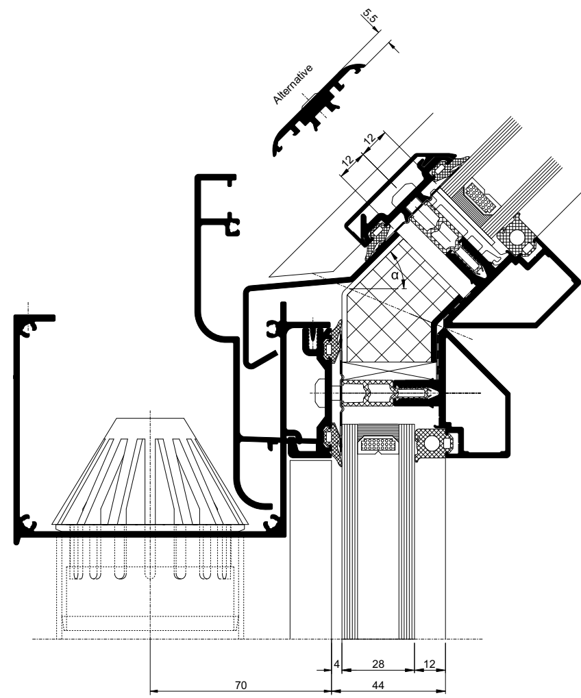
Gutter Detail
