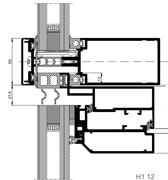
Cill Detail
