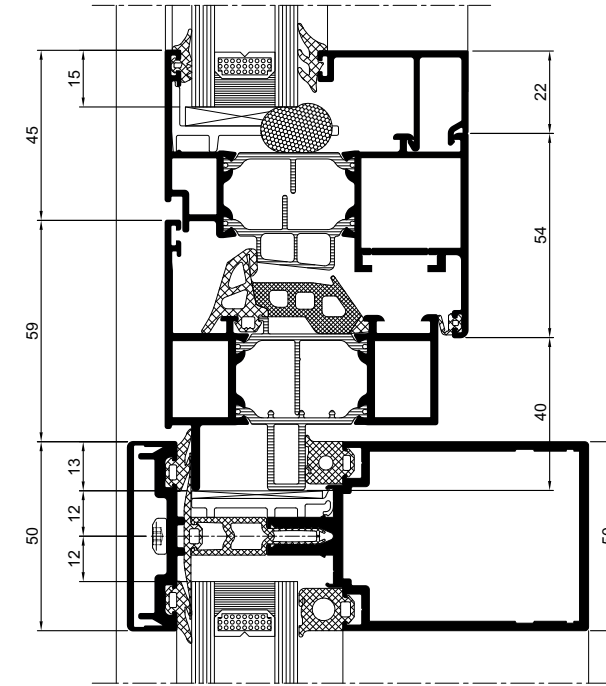
H3 06.01
