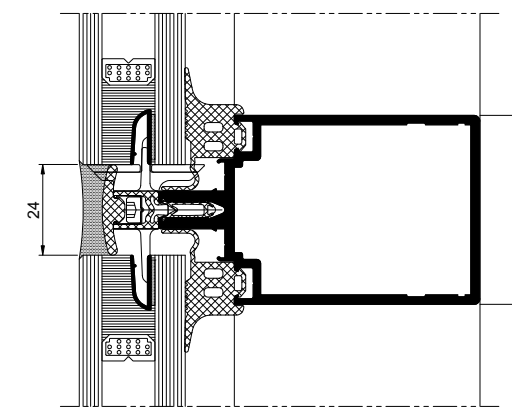
H 05.01
