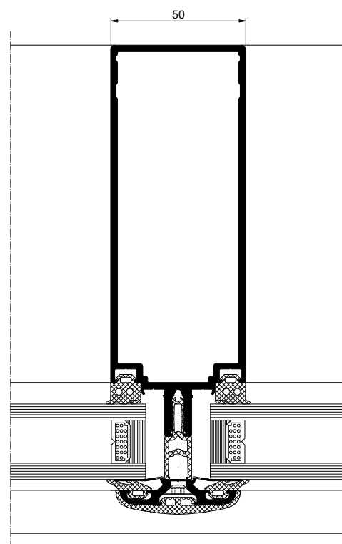
Intermediate Mullion
