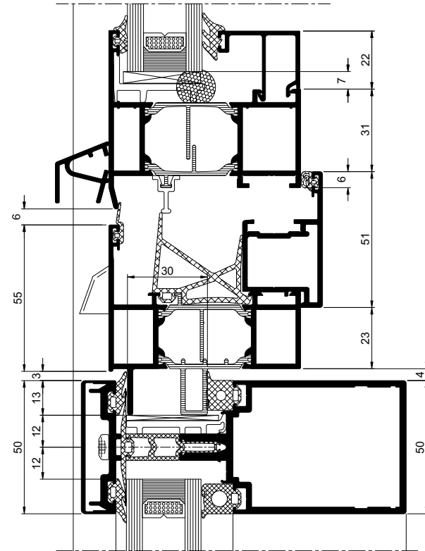
H3 07.01
