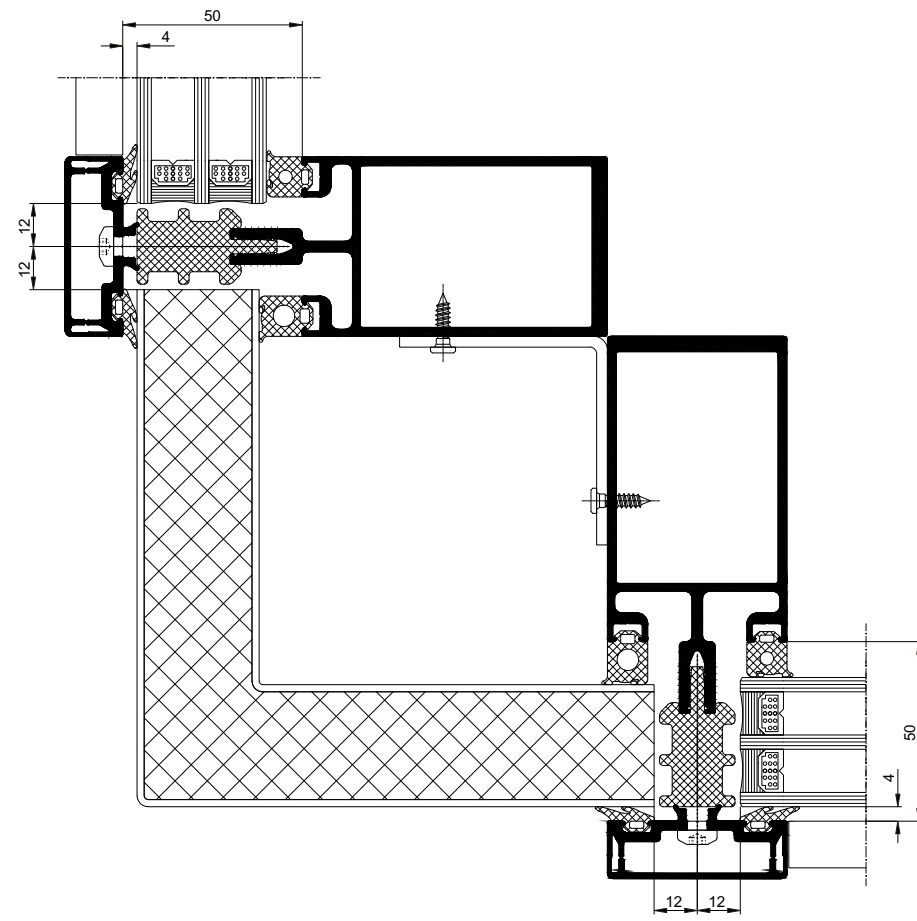
External Corner
