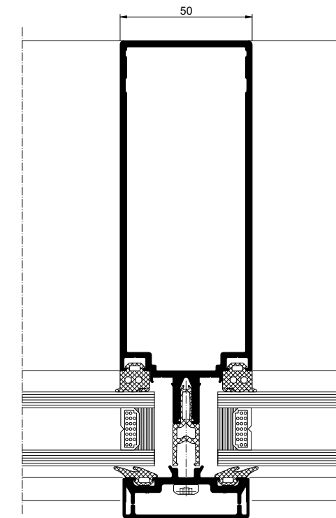
Intermediate Mullion
