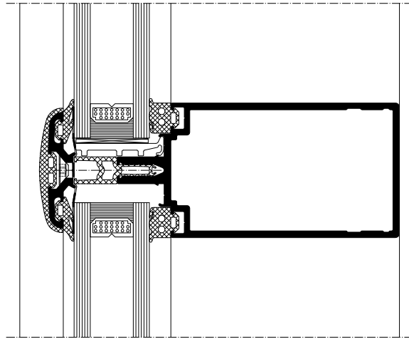
Transom Detail
