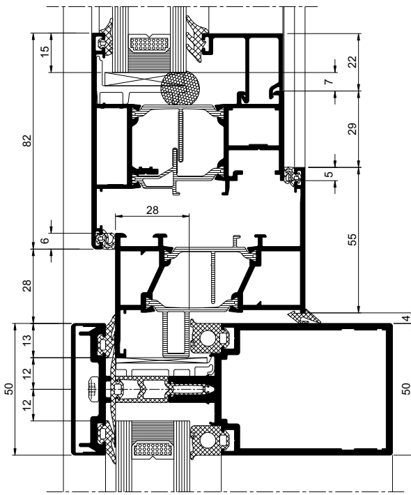
AA®100 including an AA®720 Casement
