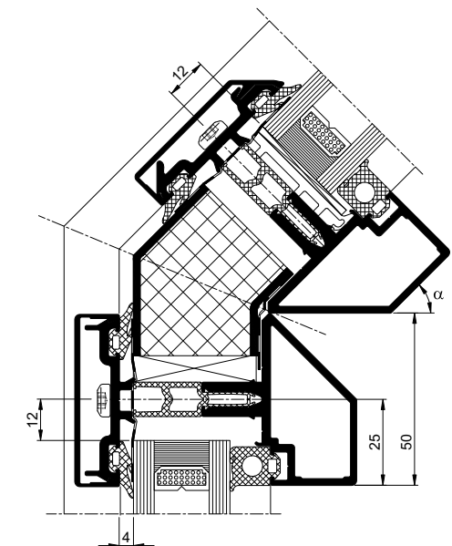
Eaves Detail (15° to 90° Pitch)
