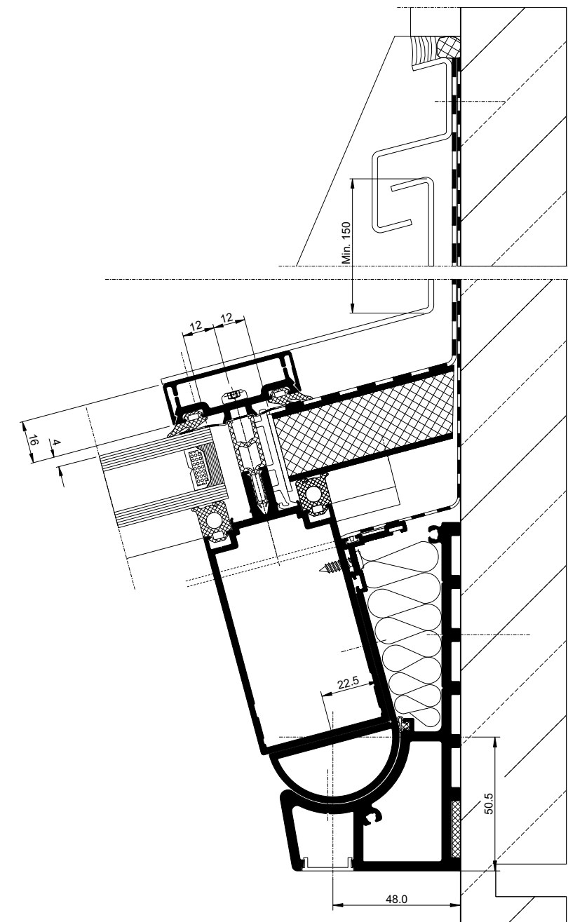
Wall Plate
