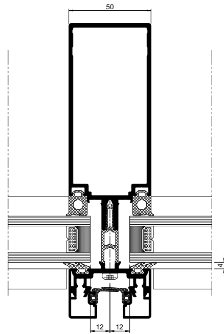
Intermediate Mullion
