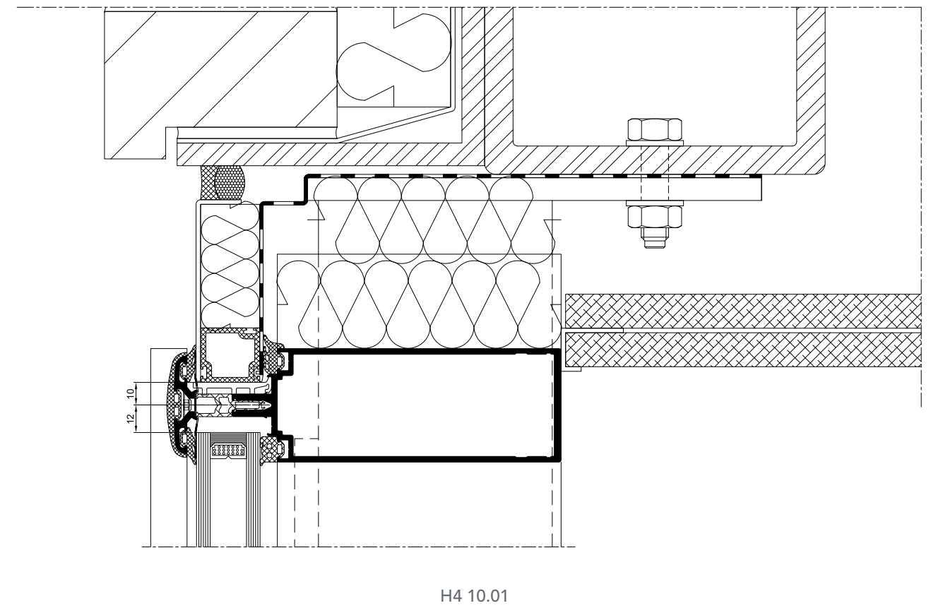
Head Detail (Generic)
