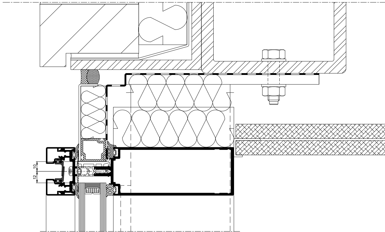
Head Detail (Generic)
