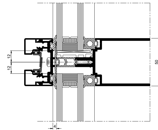
Intermediate Transom
