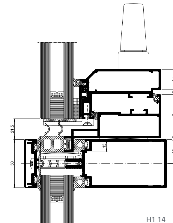
Cill Detail
